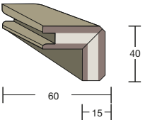
3-LAYERS STAIR NOSING RIGHT ANGLE
