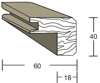
SOLID WOOD STAIR NOSING RIGHT ANGLE
