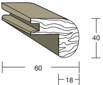
SOLID WOOD STAIR NOSING ROUNDED
